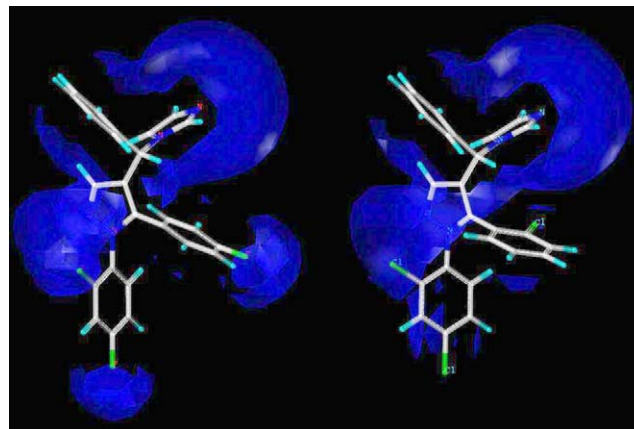
Figure 4. Isopotential contour maps for 10o (left) and 10j (right). Only negative potentials have been represented, coloured in blue. The cut has been done at -4.00 level.
