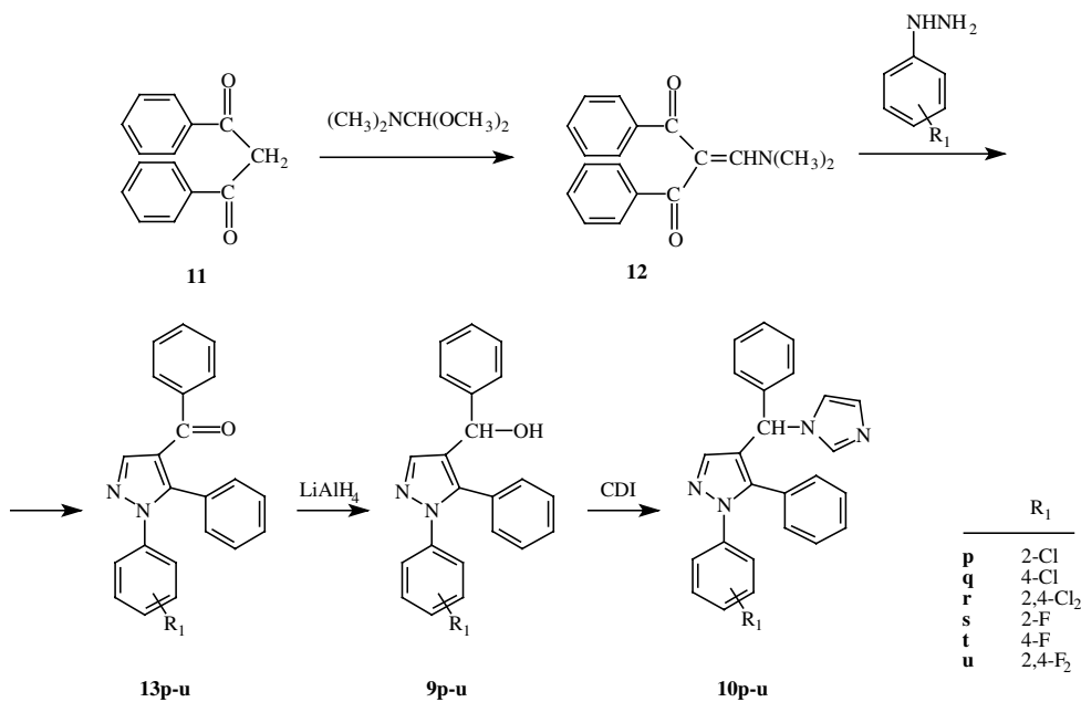
Scheme 2. Synthesis of compounds 10p–u.
