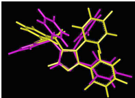
Figure 3. A superimposition of the best FlexX docking solution for 10j (magenta) and for 10o (yellow).
