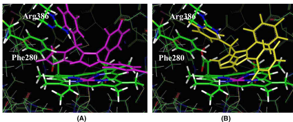
Figure 2. Binding mode proposed for 10j (A) and 10o (B) into the catalytic site of MT-CYP121. For the sake of clarity, only few amino acids of the macromolecule are displayed as sticks.
