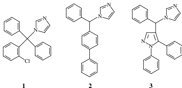
Figure 1. Structures of clotrimazole ( 1 ), bifonazole ( 2 ) and 1,5-diphenylpyrazole analogue of bifonazole ( 3 ).
