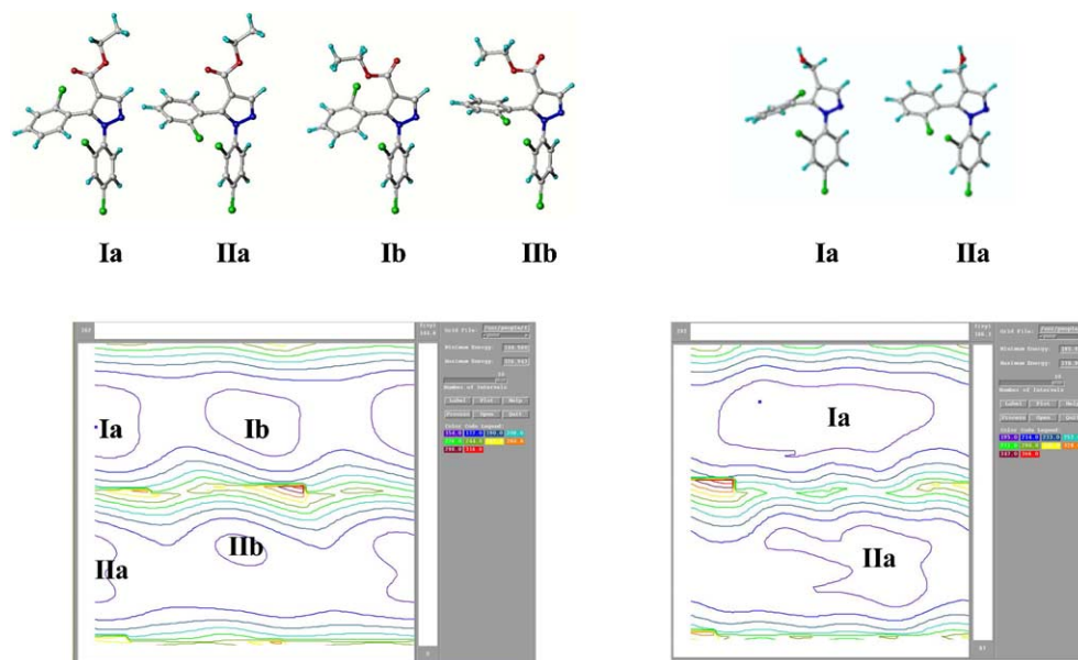
Figure 6. Ramachandran plots of compound 6j , 7j and their identified conformers. Different colours define different energetical areas. Colour code (kJ/mol): violet 154.0, dark-blue 172.0, green-blue 190, turquoise 208.0, light-green 226.0, dark-green 244.0, yellow 262.0, orange 280.0, brown 298.0, red 316.0.
