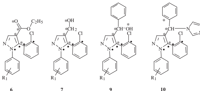
Figure 5. Torsional angles \tau_1 (*) and \tau_2 (●) selected for the conformational analysis.
