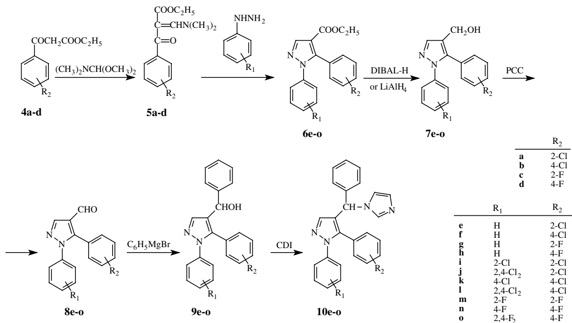
Scheme 1. Synthesis of compounds 10e–o.
